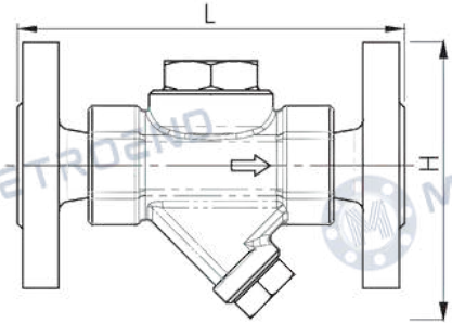
FLANŞLI / FLANGED
