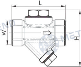
DİŞLİ / THREADED
